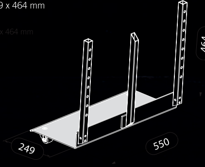
Toe plate with rollers
