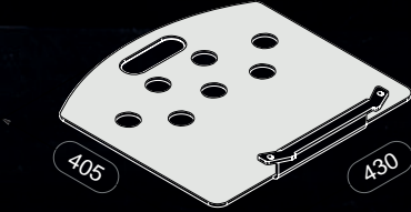
Toe plate to hook on 430 x 405 mm
