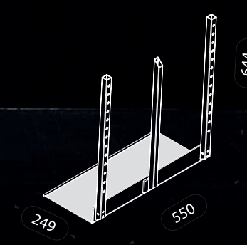
25 cm - extended beams
