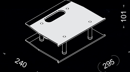
Toe plate for a laundry cart 295 x 240 x 101 mm
