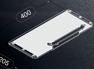
Toe plate to hook on for crates with drinks 400 x 205 mm
