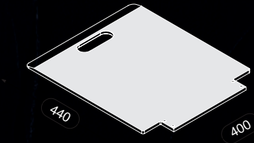
Toe plate 400 x 440 mm
