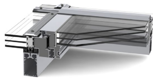
LAMILUX Ventilation Flap PR60 Variant 2
