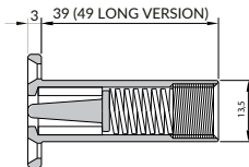
ROUNDED, STANDARD VERSION
