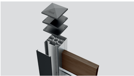
Variety of decorative post caps (pyramid, triangle or flat style) available in long-lasting colors.
